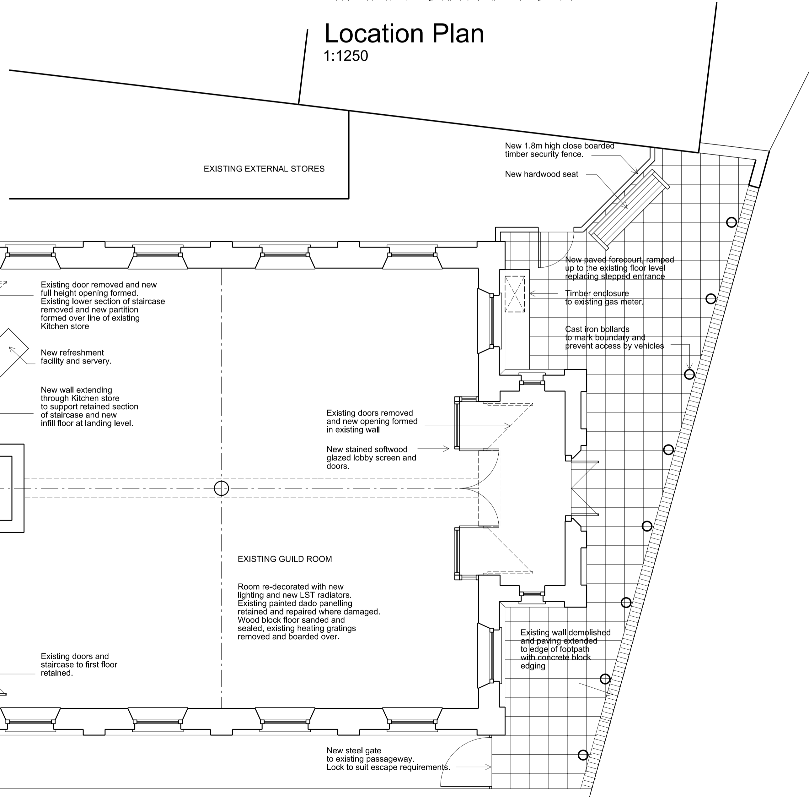
Guild Room plan as proposed
